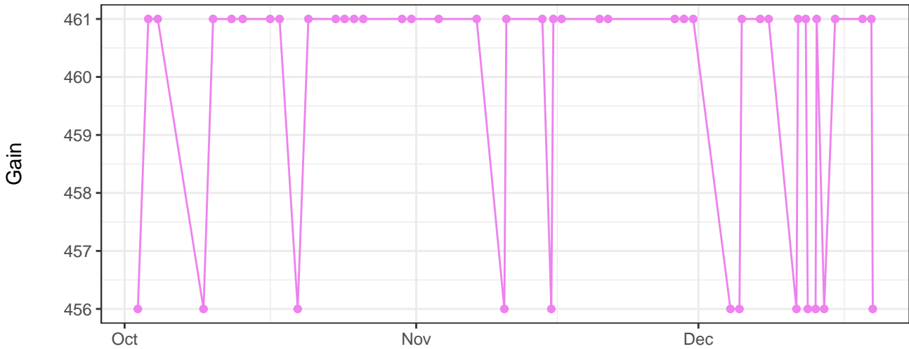
V530-A_Gain
