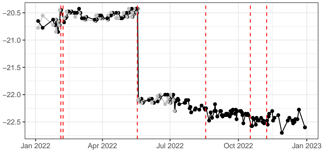
Blue_LaserDelay
