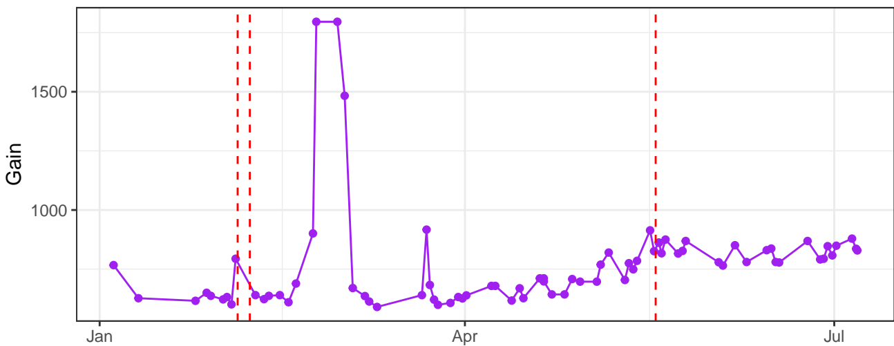
UV14-A_Gain
