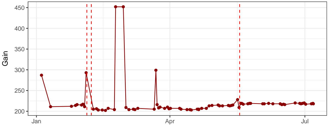
R6-A_Gain
