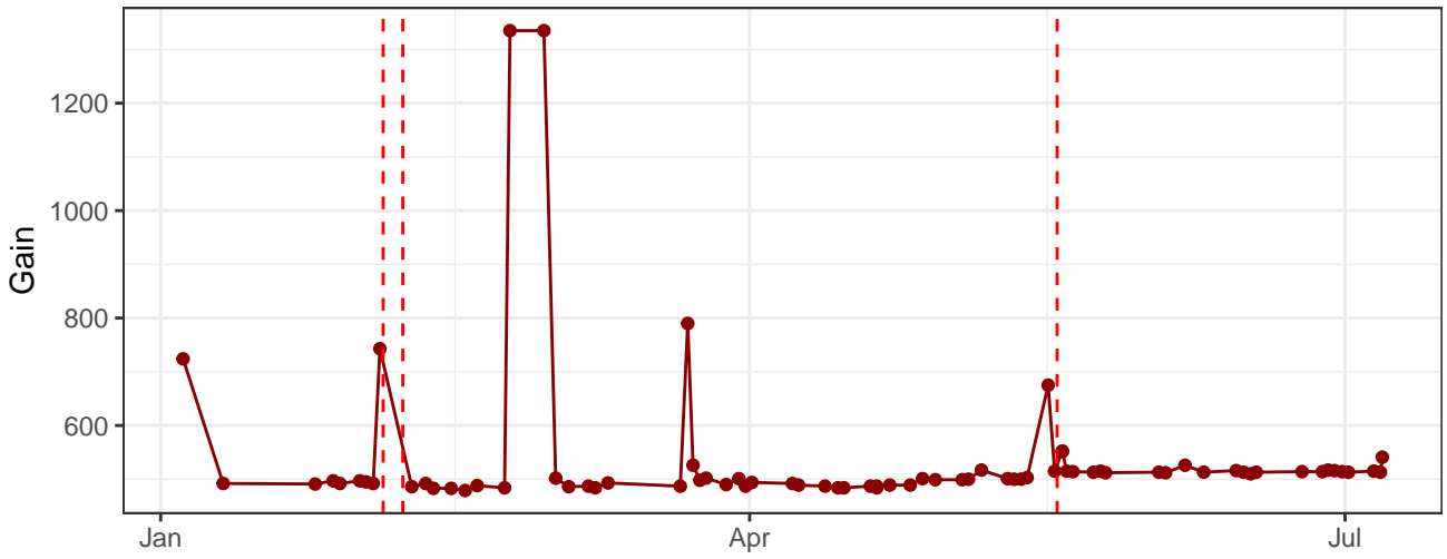
R7-A_Gain
