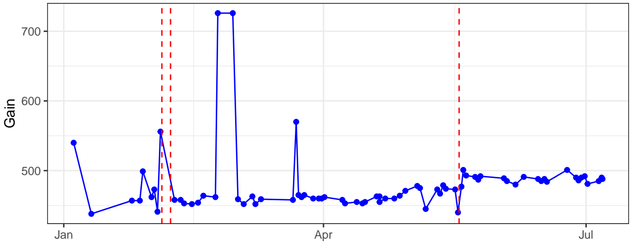
B11-A_Gain
