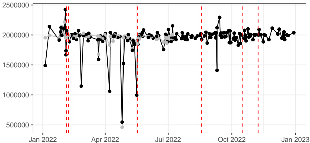
UV1-A_Gain
