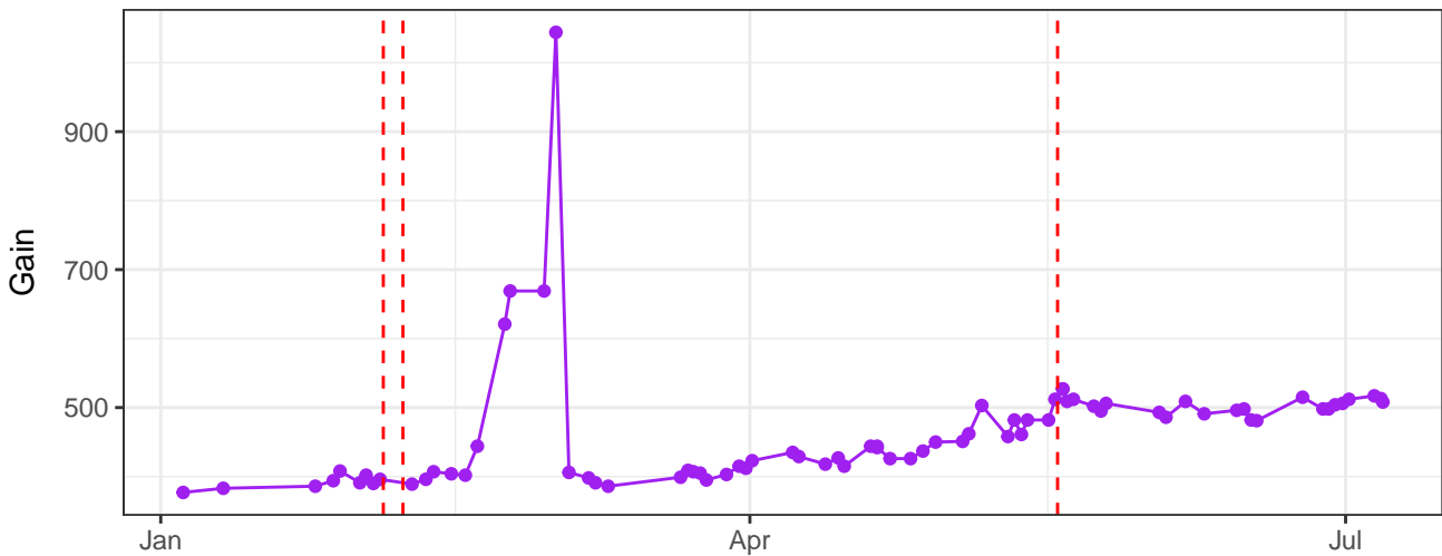
UV4-A_Gain
