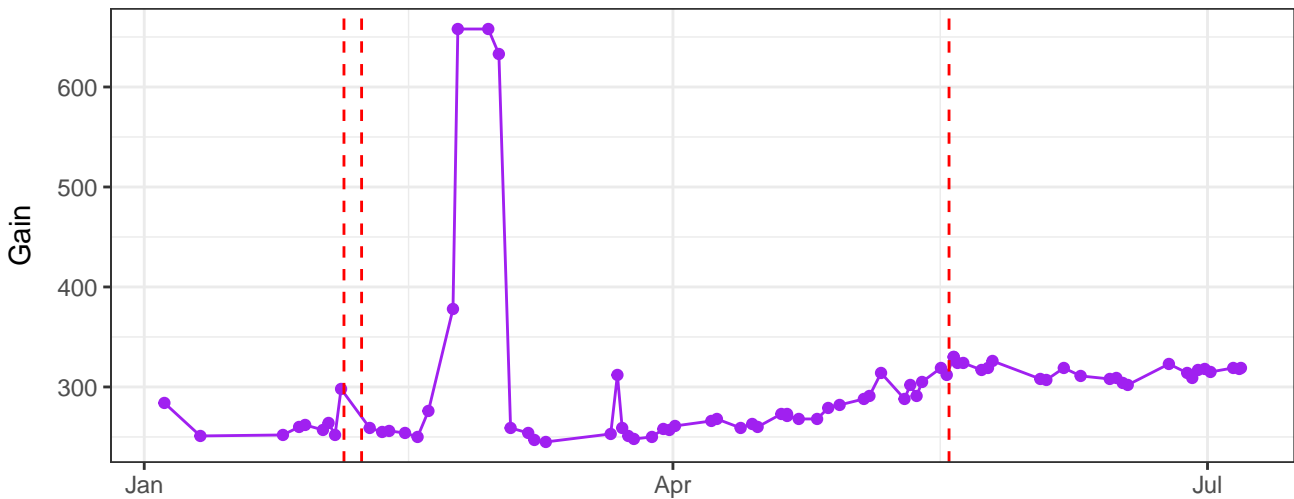
UV13-A_Gain
