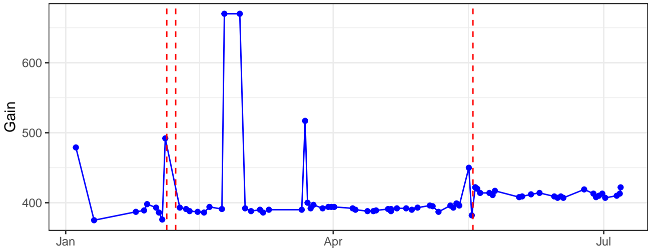
B12-A_Gain
