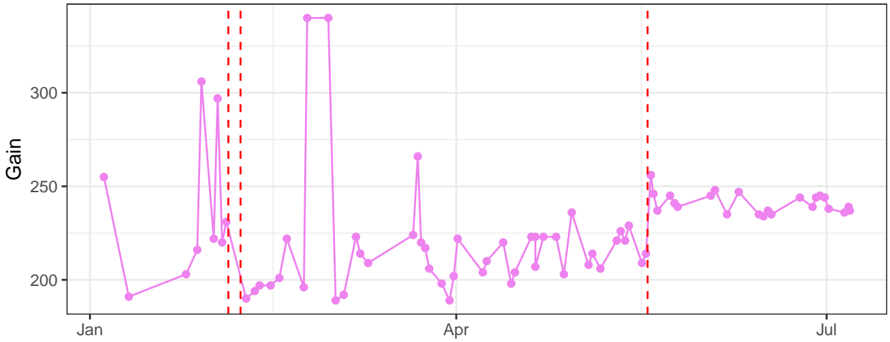
V13-A_Gain
