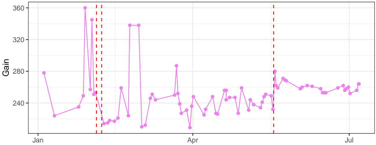
V12-A_Gain
