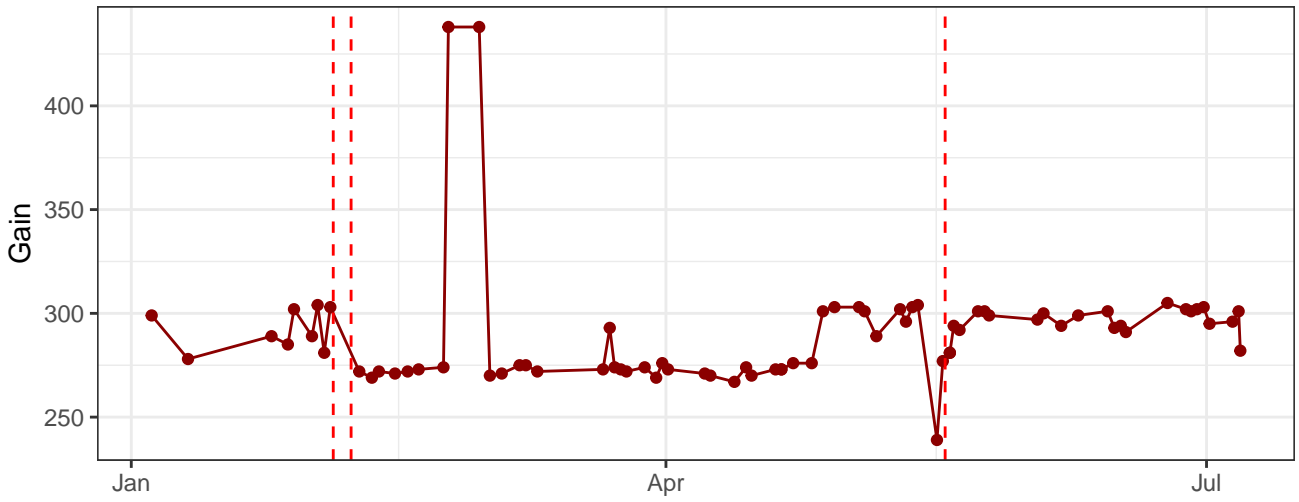
R3-A_Gain
