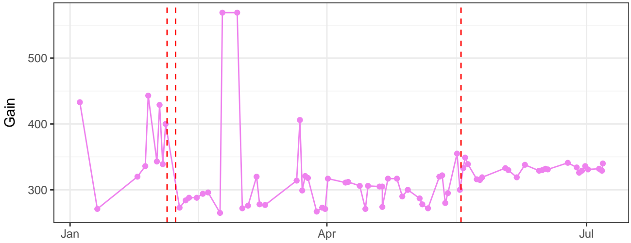
V15-A_Gain
