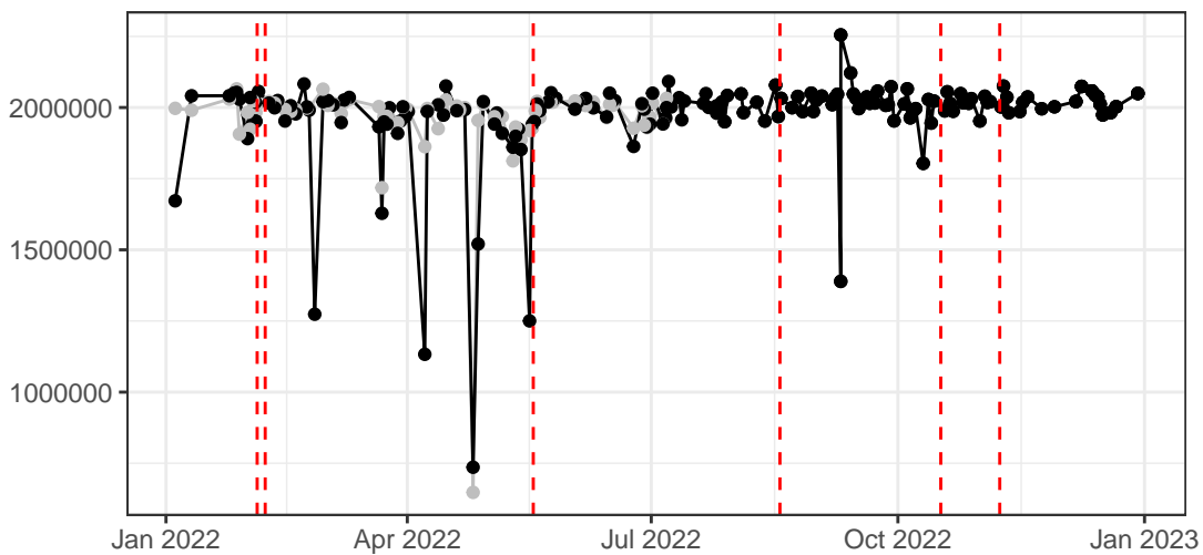
FSC-H
