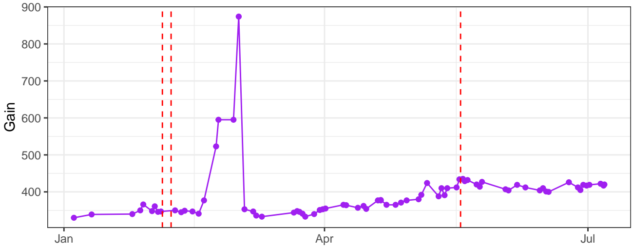
UV10-A_Gain
