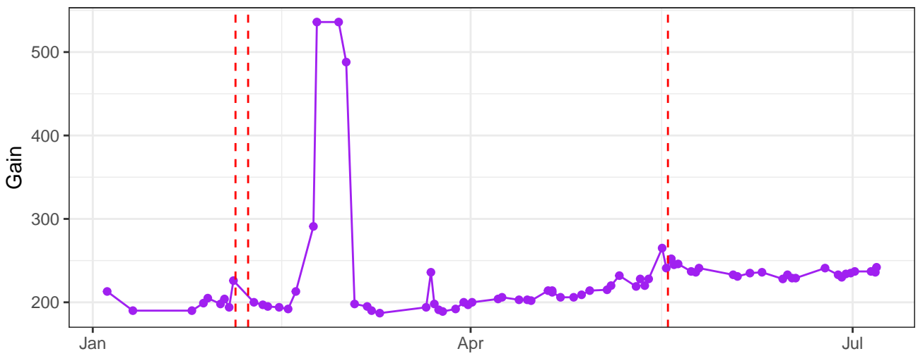
UV11-A_Gain
