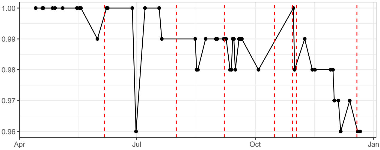
YellowGreen_AreaScalingFactor
