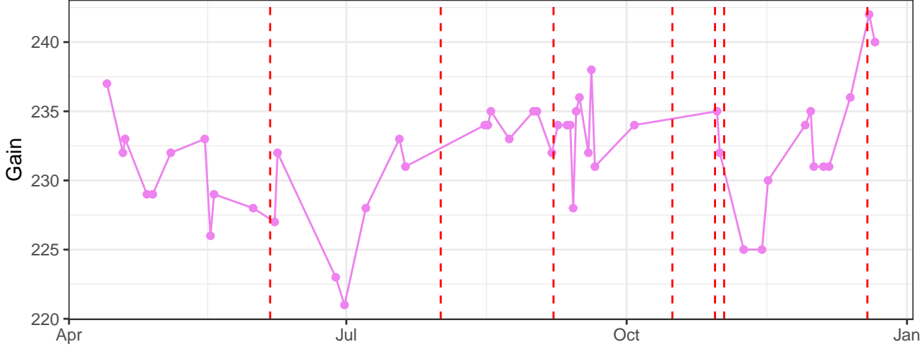
V7-A_Gain
