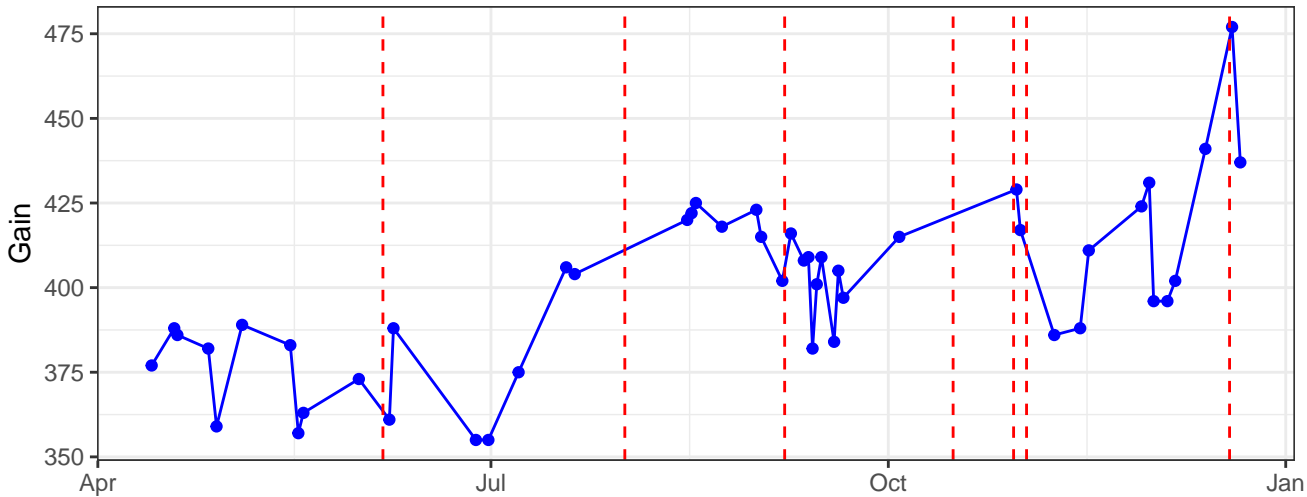
B5-A_Gain
