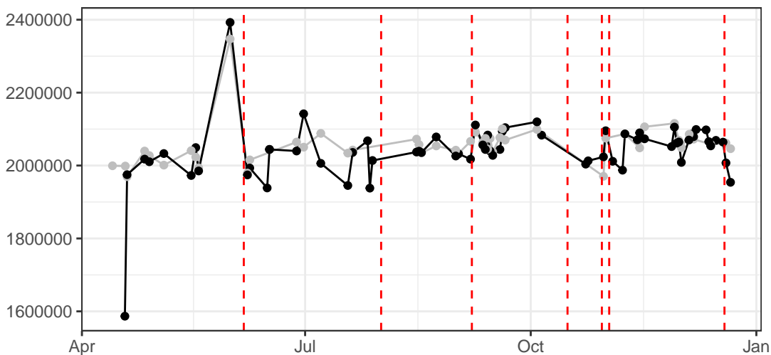
SSC-H
