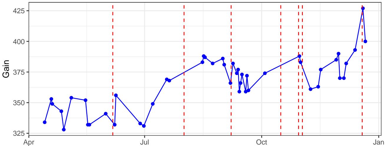
B6-A_Gain
