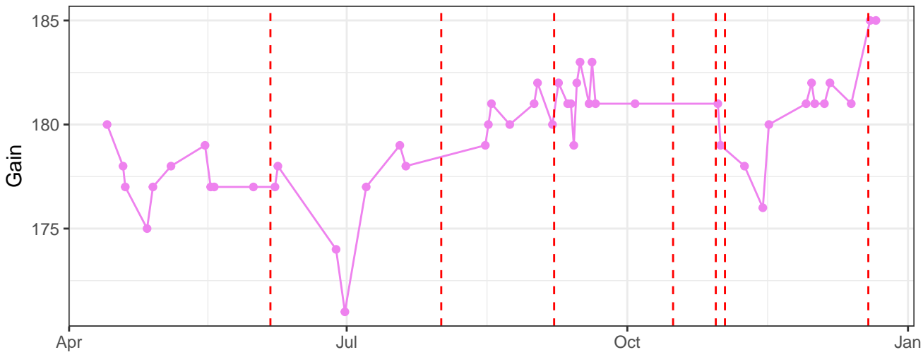
V6-A_Gain
