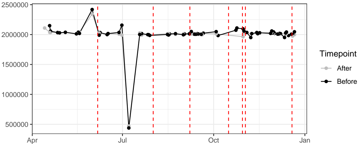
FSC-H
