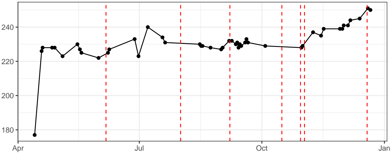
SSC-B-A_Gain
