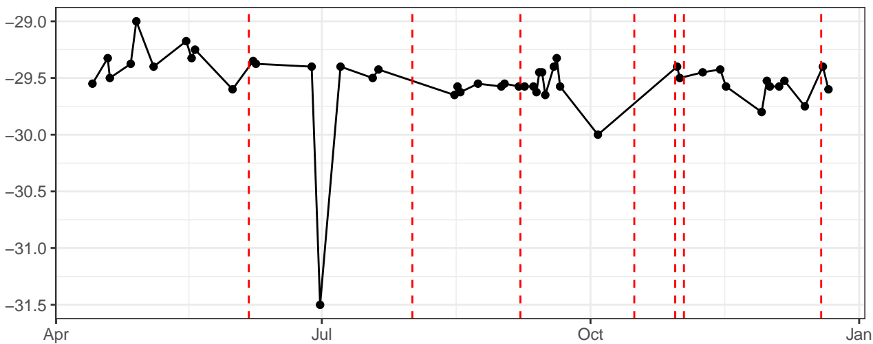
UV_AreaScalingFactor
