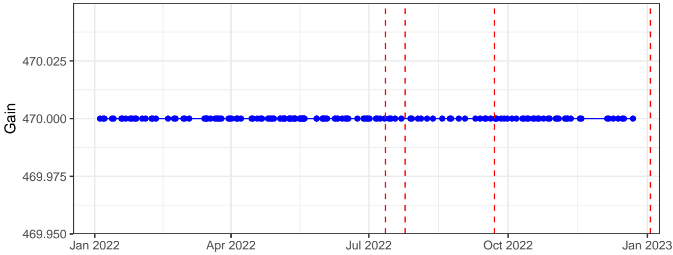
B695-A_Gain
