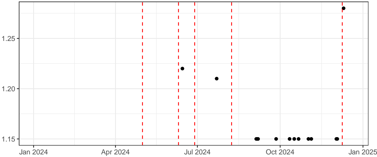
Red_AreaScalingFactor
