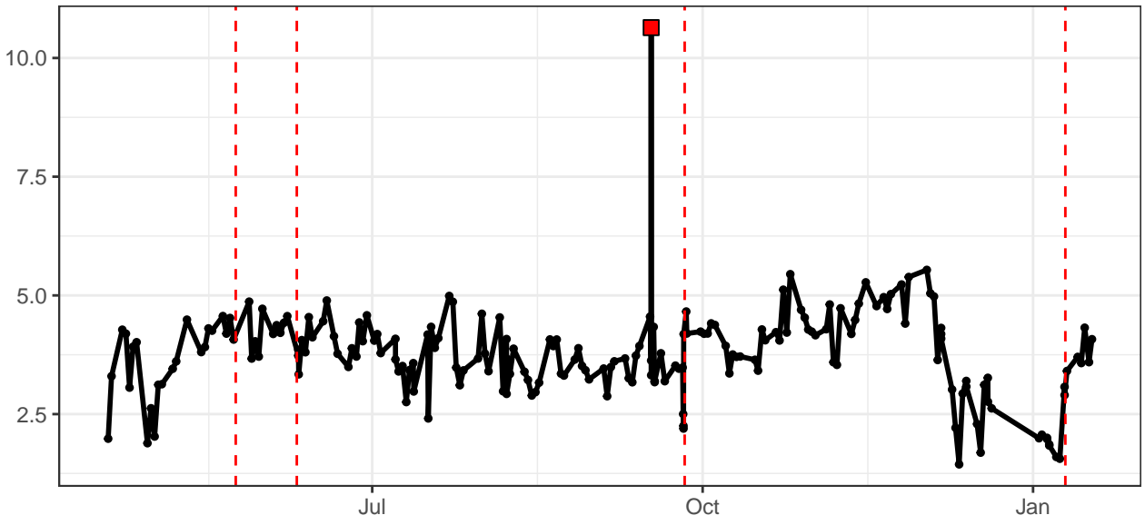
SSC-B-% rCV
