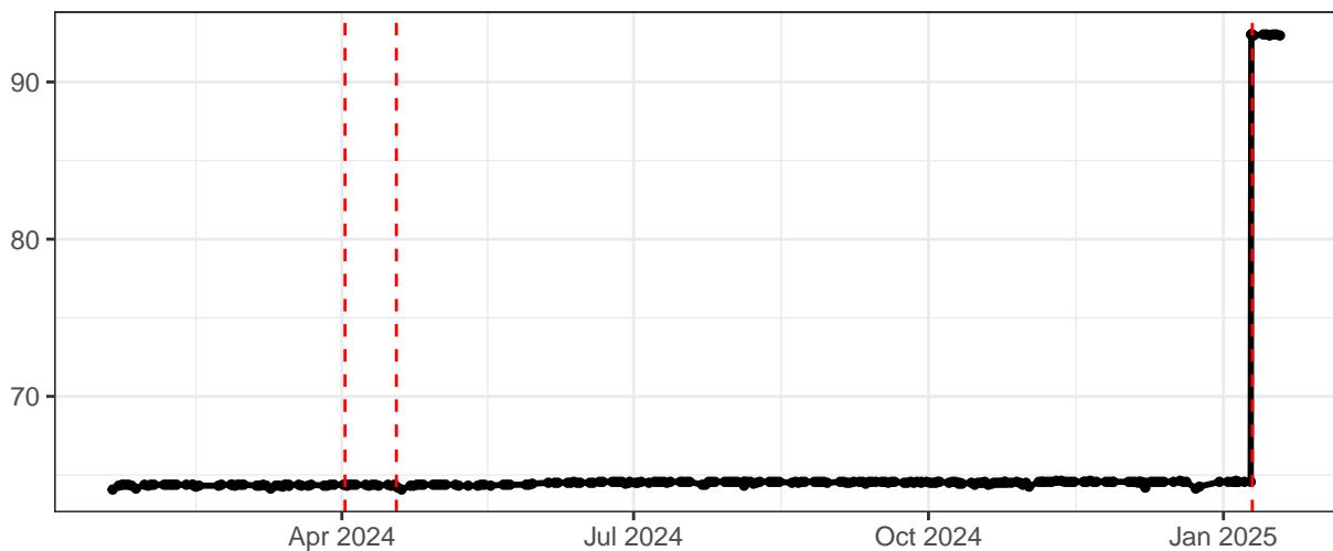
Blue-Laser Power
